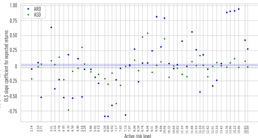
Regression coefficients of ARD and ASD according to the last specification in (3) across all 49 active risk groups. Dotted lines represent the average coefficients.
