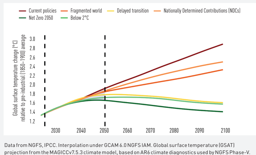
Figure 1. Global mean temperature scenario trajectories
